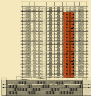
WEST FAÇADE
